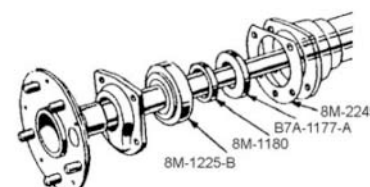
FRONT WHEEL PARTS - TYPICAL
